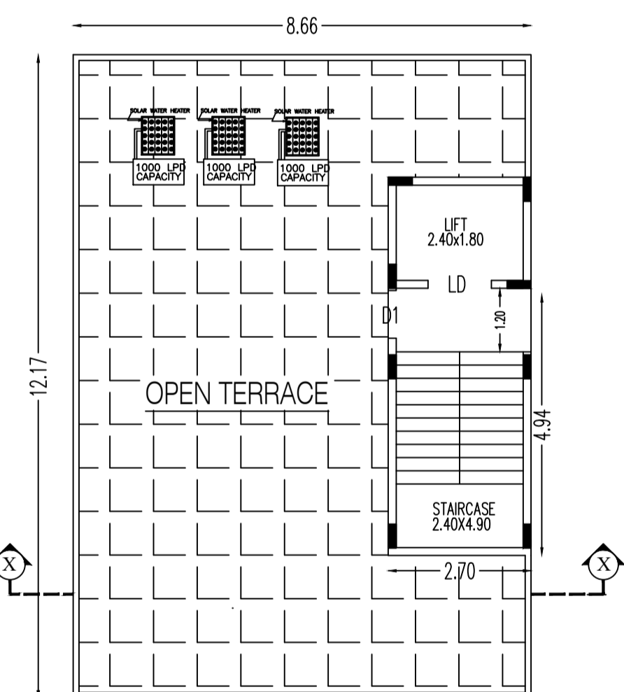
PROPOSED TERRACE FLOOR PLAN
