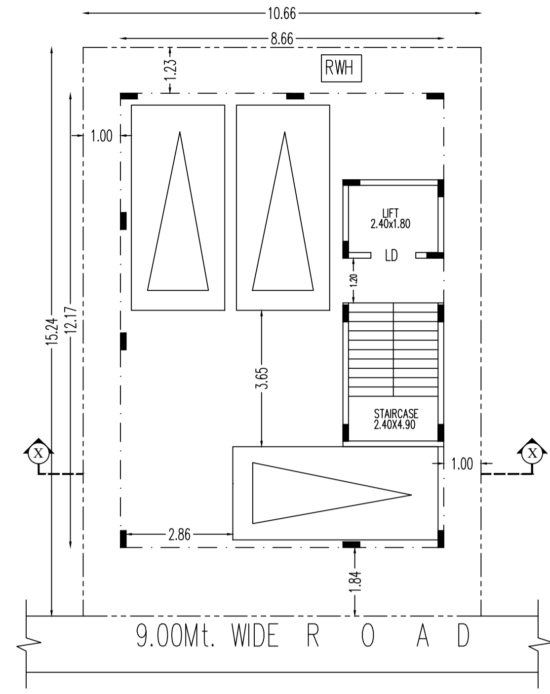
PROPOSED STILT FLOOR PLAN
