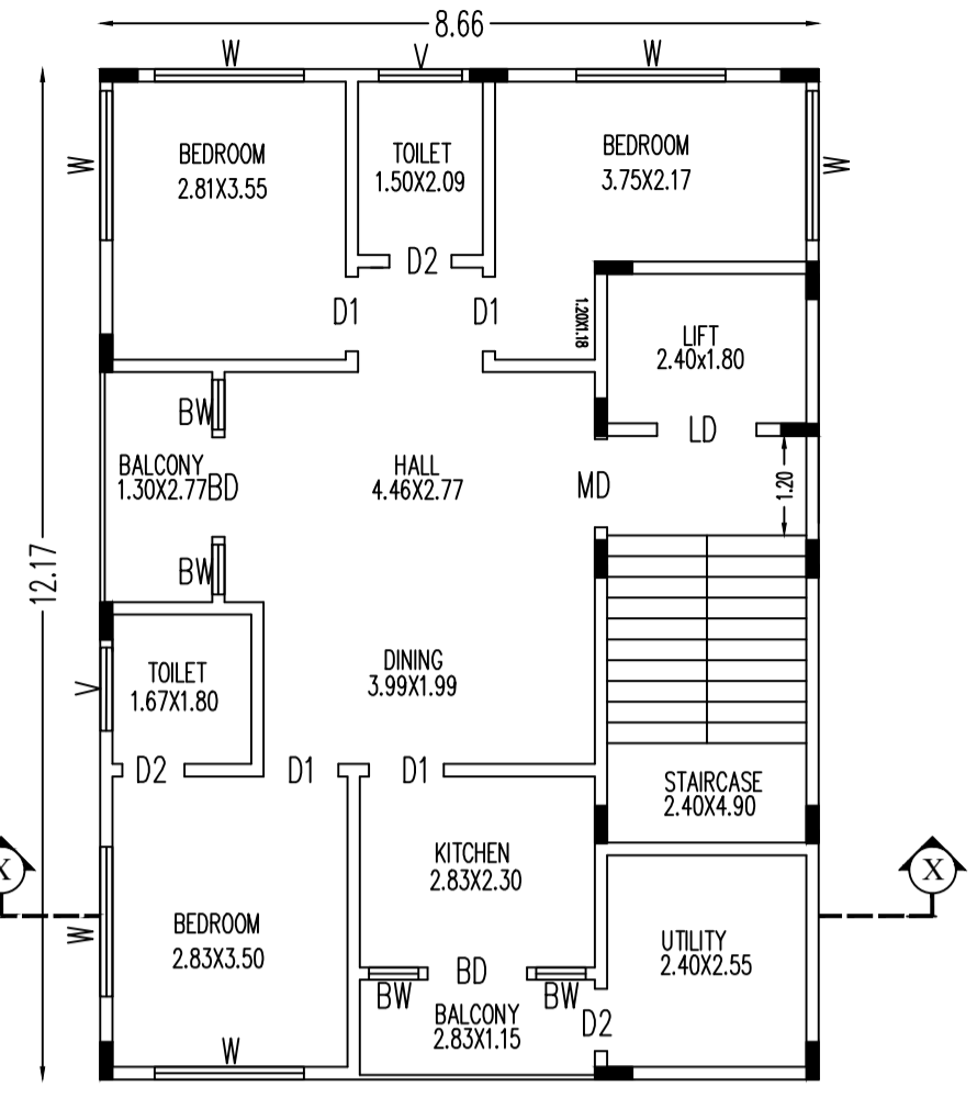
PROPOSED TYPICAL GROUND, FIRST & SECOND FLOOR PLAN
